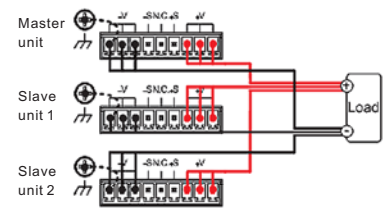
Parallel Connection
